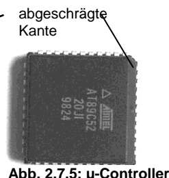
Abb. 2.7.5: \mu -Controller
