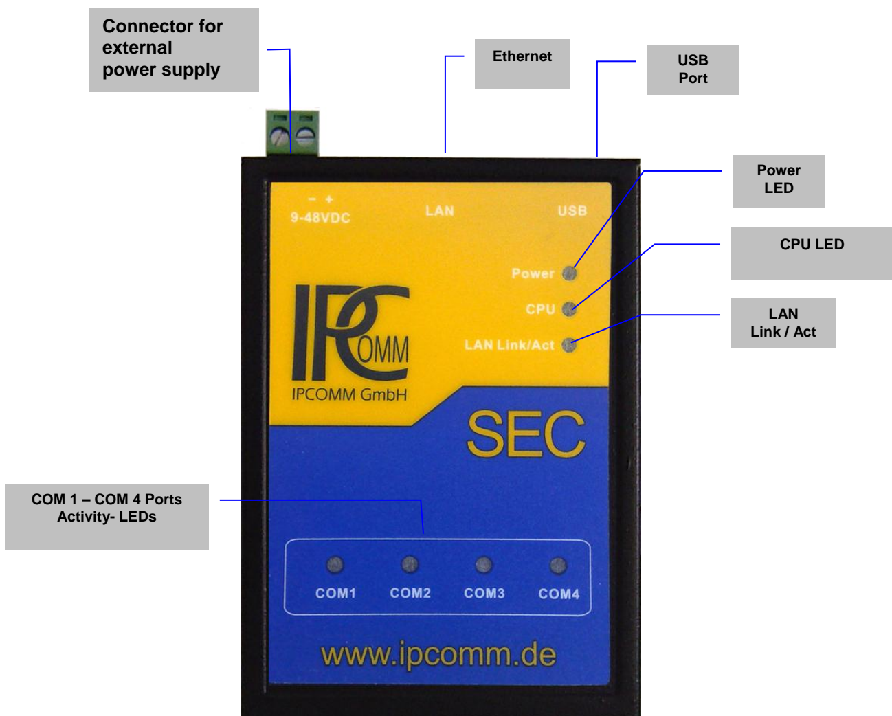
Figure 1: SEC2 front view
