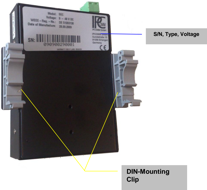
Figure 4: SEC2 rear view
