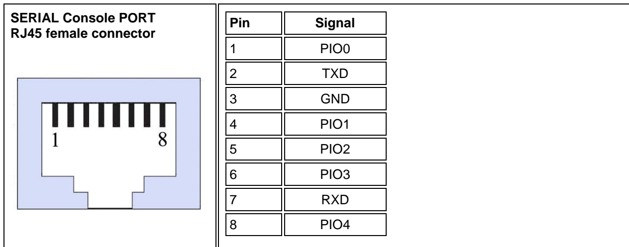
Figure 8: Pin assignment of RJ45 interface of serial console port
