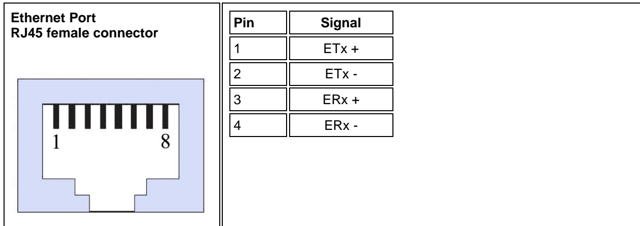
Figure 7: Pin assignment of Ethernet RJ45 interface
