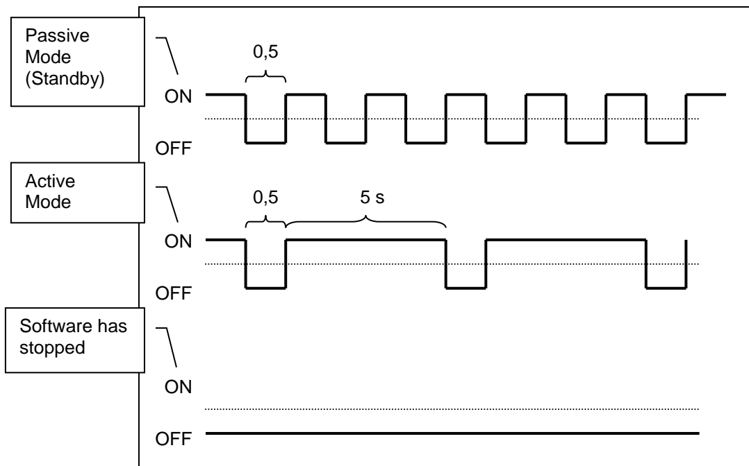
Figure 11: CPU-LED indications
