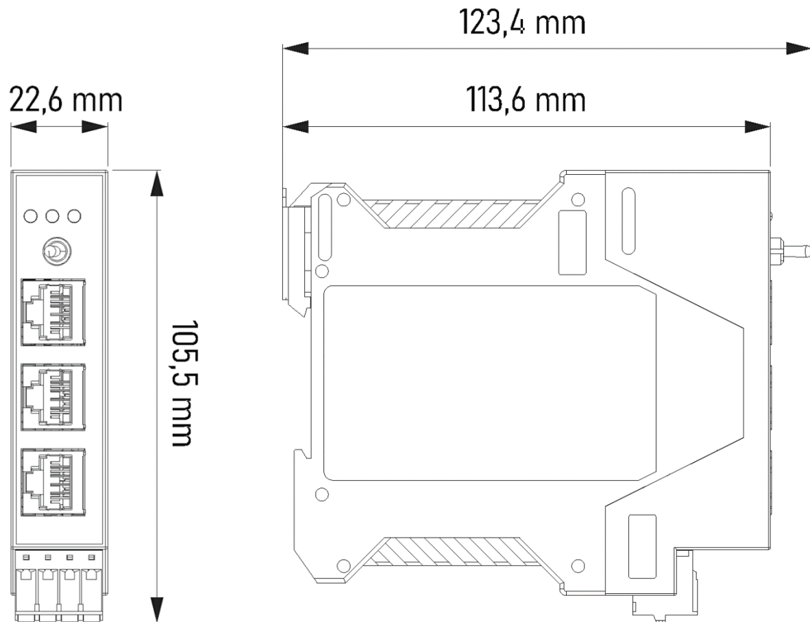
Figure 12: Dimensions – ERM1
