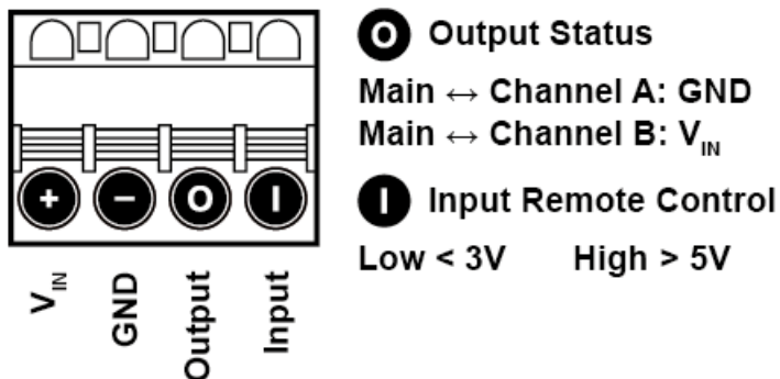
Figure 4: Digital I/O
