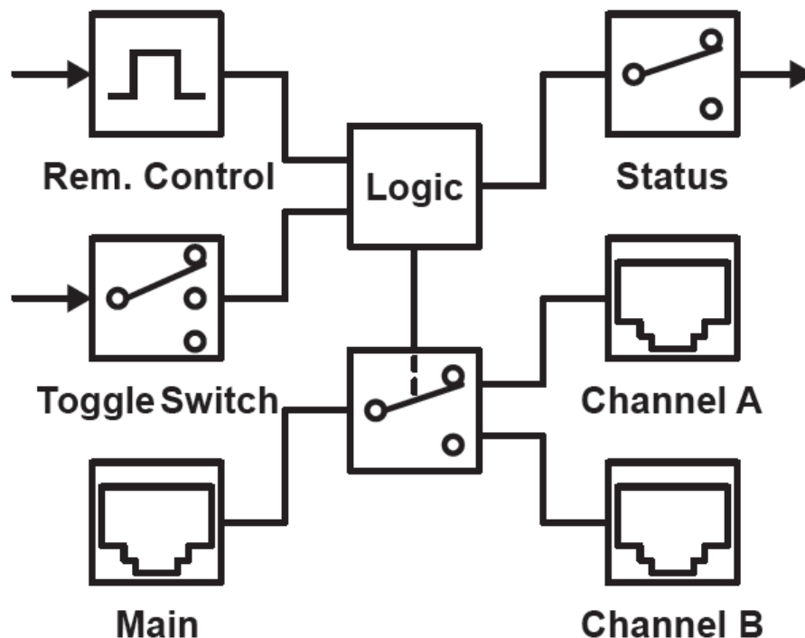
Figure 5: Control logic
