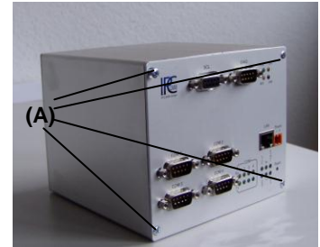
Fig. 2.5.9 Tighten the front panel screws (A).
